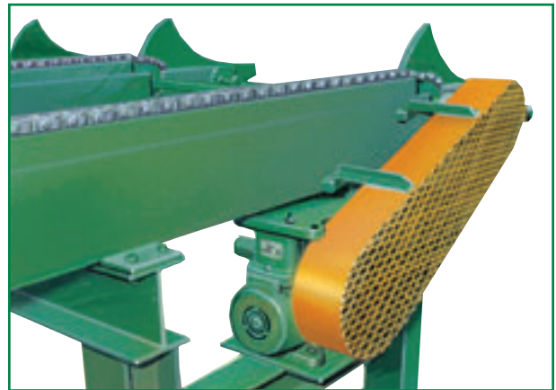
Drive shown is worm gear reducer with hydraulic motor. Optional electric motor and worm gear reducer available.
